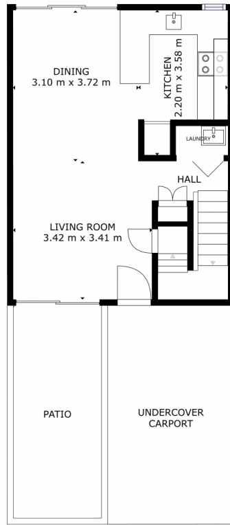
FLOOR 1
